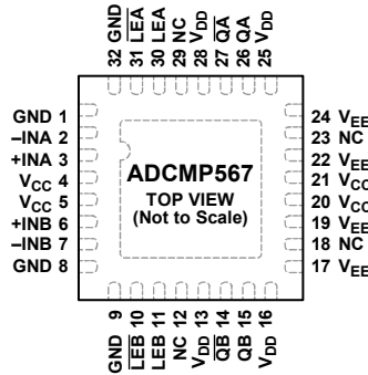
Figure 2. ADCMP567 Pin Configuration
