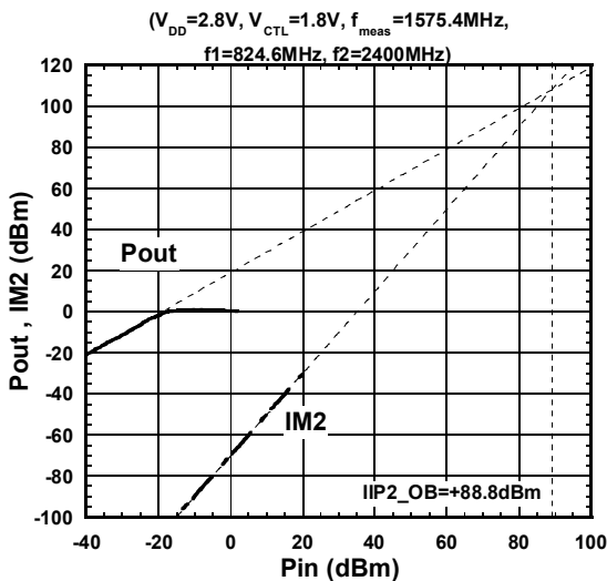
Out-of-band IIP2
