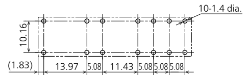
Recommended PC board pattern ( BOTTOM VIEW )
