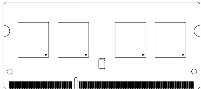
Figure 1: 204-Pin SODIMM (R/C B2, B4)
