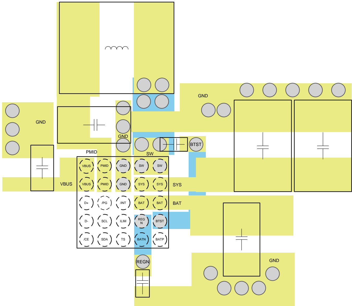
Figure 92. PCB Layout Example
