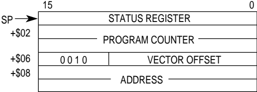
Figure B-5. Six-Word Stack Frame, Format $2
