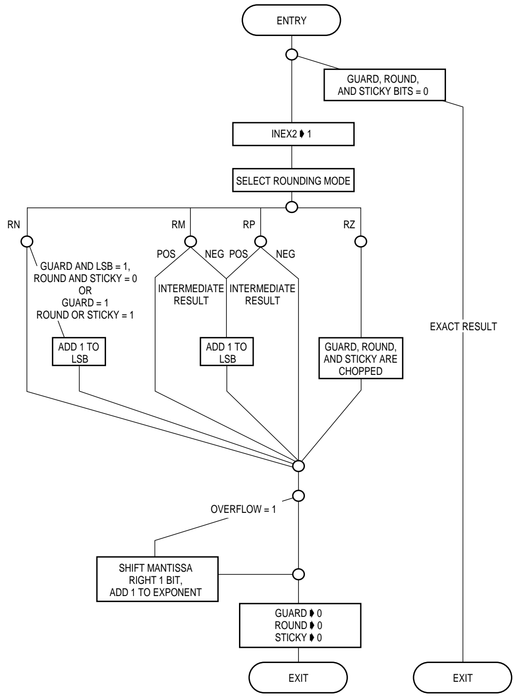
Figure 3-2. Rounding Algorithm Flowchart
