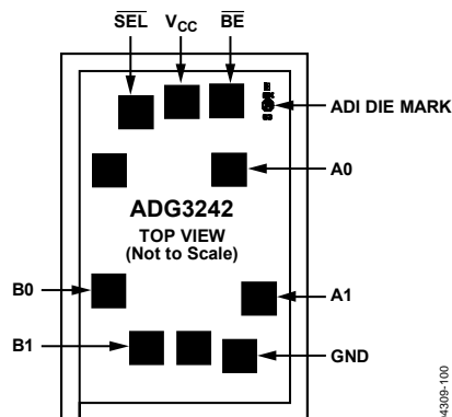
Figure 3. Die Pad Configuration (Die size: 550 μm × 820 μm)
