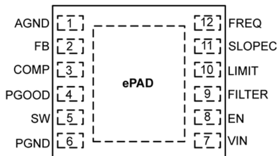
12-Pin 3mm x 3mm MLF ® (ML) (Top View)
