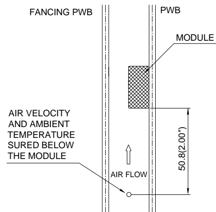
Figure 19: Wind tunnel test setup
