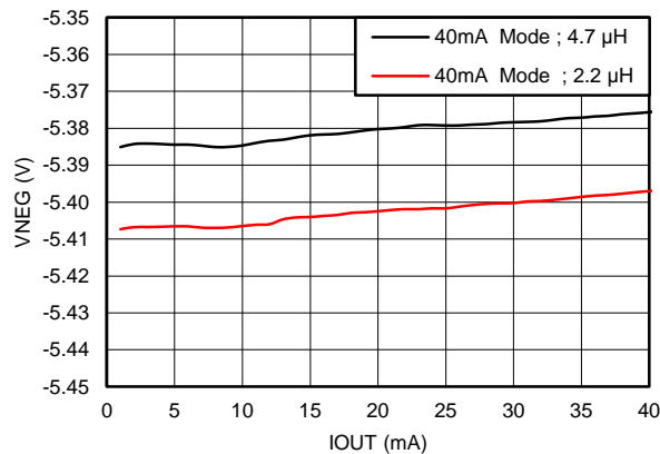
Figure 46. Load Regulation
