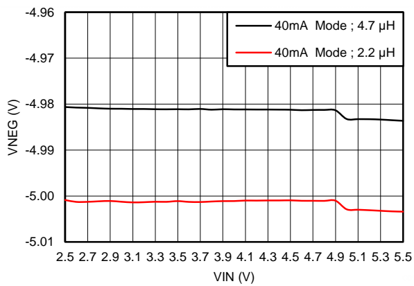
Figure 49. Line Regulation
