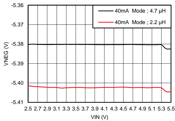
Figure 50. Line Regulation
