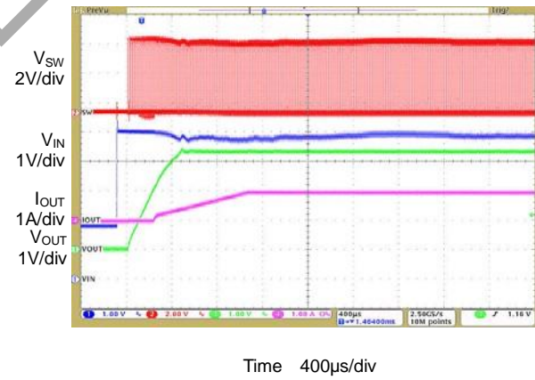
Figure 31. Soft Start Function ( V_{IN}=5V , V_{OUT}=3.3V , I_{OUT}=1A )
