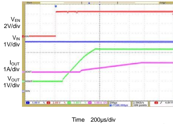
Figure 28. EN Pin L to H ( V_{IN}=5V , V_{OUT}=3.3V , I_{OUT}=1A )
