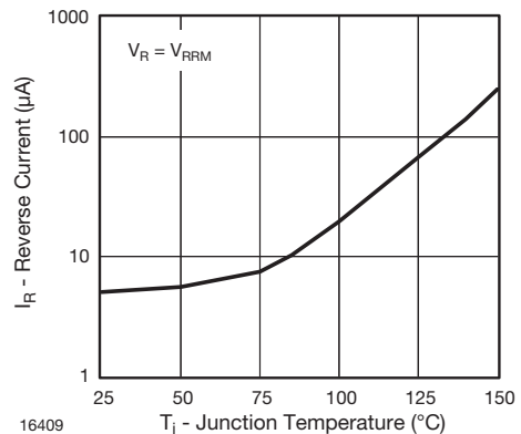
Fig. 4 - Reverse Current vs. Junction Temperature
