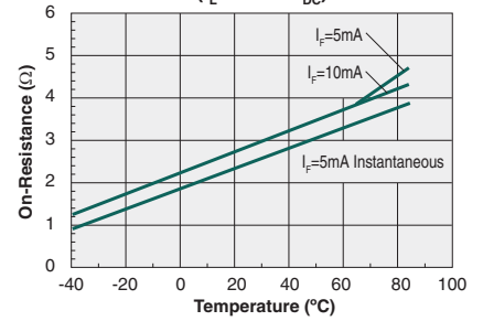
Typical On-Resistance vs. Temperature AC/DC Configuration ( I_L=350\text{mA}_{DC} )
