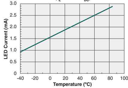
Typical I_F for Switch Dropout vs. Temperature ( I_L=200\text{mA}_{DC} )
