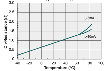
Typical On-Resistance vs. Temperature DC-Only Configuration ( I_L=350\text{mA}_{DC} )
