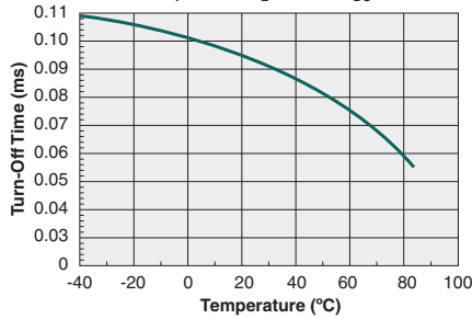
Typical Turn-Off Time vs. Temperature ( I_F=5\text{mA} , I_L=200\text{mA}_{DC} )
