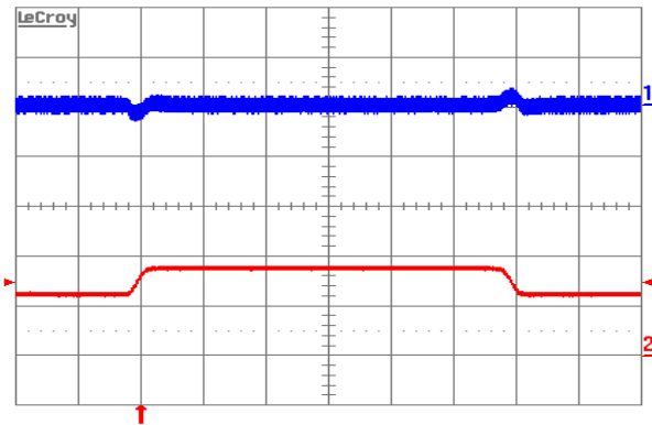
Figure 8. Output voltage response to load current step-change (12.5A–18.75A–12.5A) at V_{in} = 48\text{ V} . Top trace: output voltage (100mV/div.). Bottom trace: load current (10A/div.). Current slew rate: 0.1\text{ A}/\mu\text{s} . C_o = 1\mu\text{F cer} + 10\mu\text{F tant} . Time scale: 0.2ms/div.
