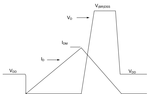
Figure 17. Unclamped inductive waveform
