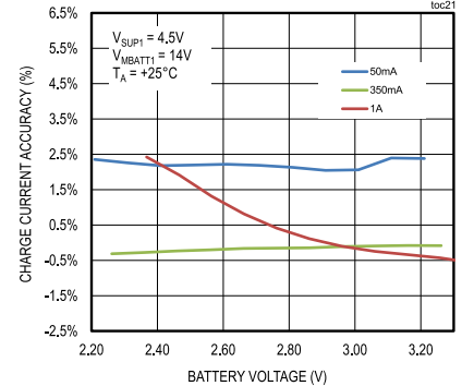
CHARGE CURRENT ACCURACY vs. BATTERY VOLTAGE
