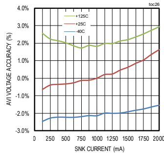
AVI VOLTAGE ACCURACY vs. SNK CURRENT
